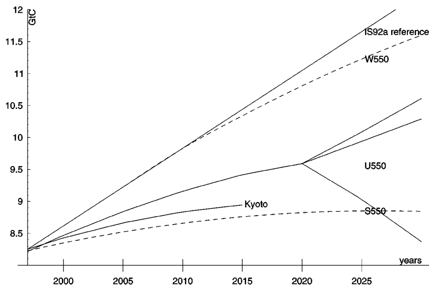
Figure 2. Global CO 2 emissions pathways consistent with long-term stabilization of concentration. The S550 and W550 trajectories illustrate two extreme attitudes with respect to early action. The U550 curve illustrates a sequential decision-making strategy. It assumes that the 550 ppm target is only an expected value, to be revised to 450, 550 or 650 ppm in 2020; and it minimizes reduction costs using the DIAM model [1, p. 707].
