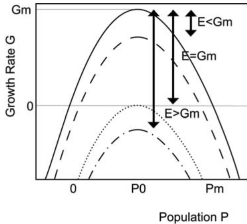
Figure 1. Basic relation for the didactic model to explain the qualitative modeling approach. If subject to a constant withdrawal E , the U-shaped relation between the population P and the growth rate G gives rise to three different types of behavior. Starting from the climax state P = P_m , the population either stabilizes at a level beyond P_0 , if the withdrawal is less than G_m (dashed line) or right at P_0 if E = G_m (dotted line). In case of E > G_m , the population finally vanishes (dash-dotted line).
