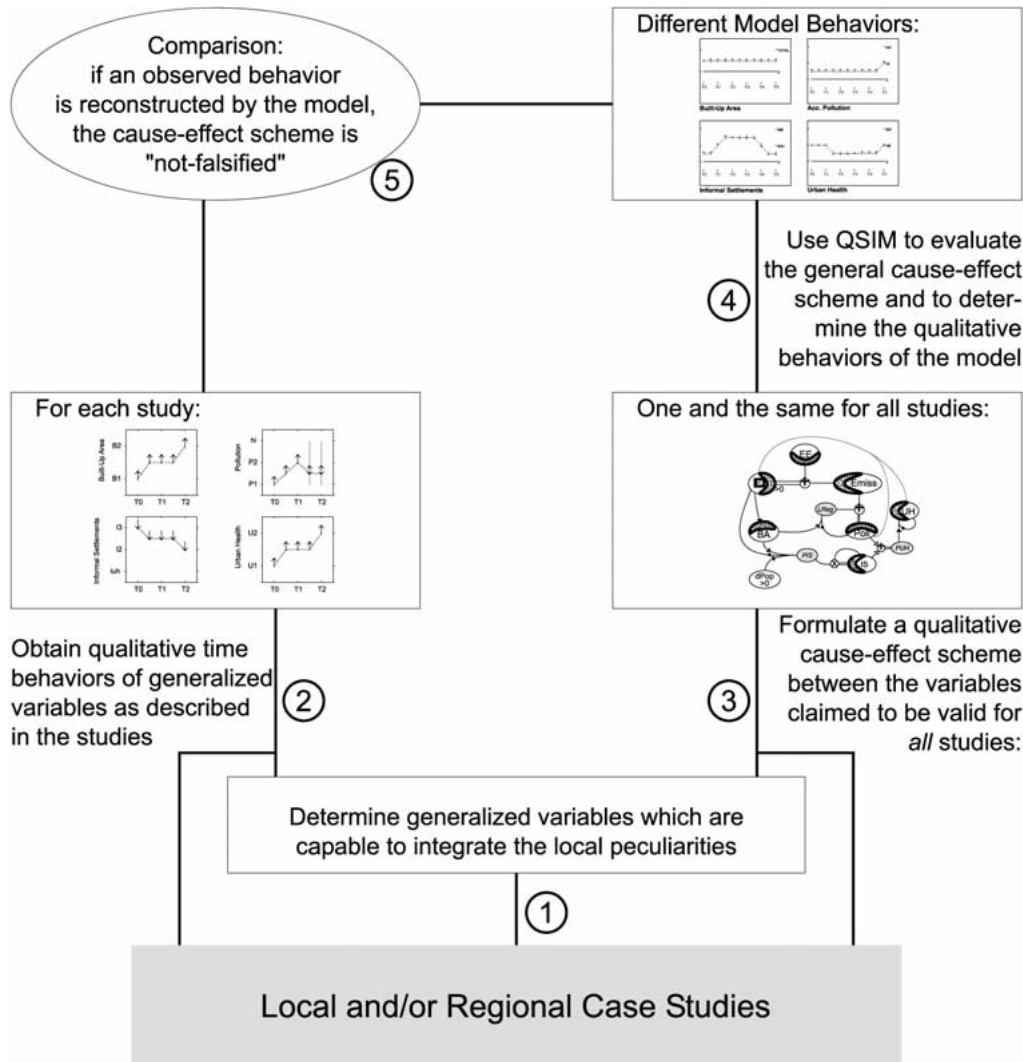
Figure 3. Case-study integration scheme.
