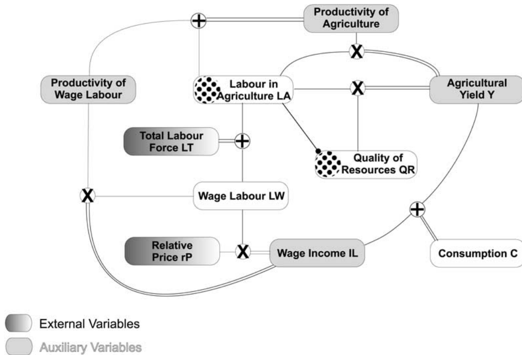
Figure 4. Qualitative model for integration of the case studies. The different lines and symbols encode actual realizations in the qualitative model, i.e., dotted areas: Temporal change of the variable; “+” qualitative addition; “x” qualitative multiplication; “—•” monotonously decreasing relation (see appendix).
