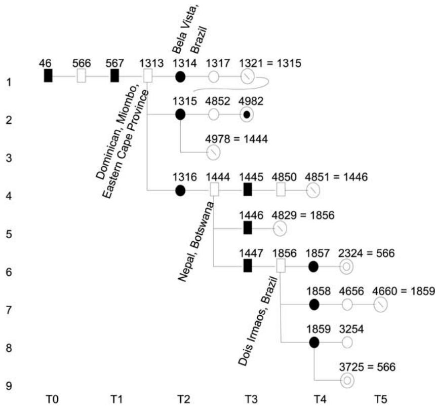
Figure 5. Behavior tree of the qualitative model for smallholder agriculture as specified in figure 4, representing the entire set of possible solutions. In addition to the symbols already introduced in section 3, the transition symbol \odot is used to indicate that the behavior continues at another node in the tree, given by the number on the right hand side of the identity indicated at the transition point. For example, the state S-1321 in the first behavior is identical to the state S-1315 in the second. Thus the first behavior is not truncated, but continues as the dashed line indicates it. The initial condition (S-46) is chosen such that – as is indicated by the labels bearing the names of the study regions and as discussed in more detail in section 5.5 – the recent history in all regions is part of the tree.
