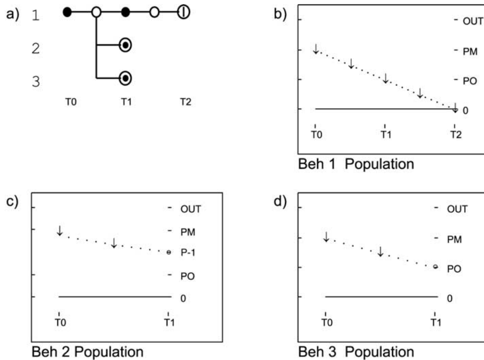
Figure 2. Behavior tree (a) and qualitative behaviors (b)–(d) for the variable “Population” of the simple didactic model for a general logistic growth of the population dynamics. Note that in figure 2(c) a new landmark is introduced by QSIM itself, denoting the final value of the population at time T1 . Further discussion see in text.
