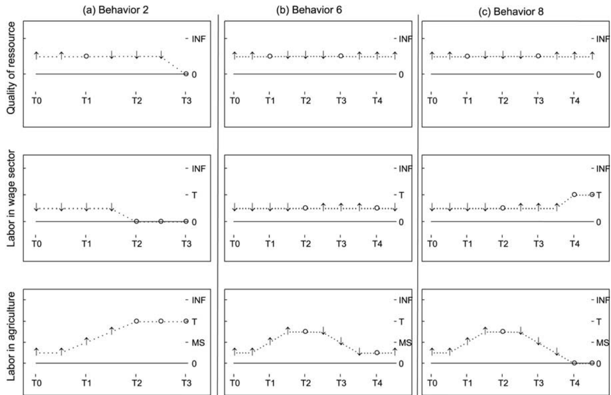
Figure 6. Qualitative time-plots for three out of nine behaviors. The behavior numbers on top refer to the behavior tree in figure 6. For a detailed discussion see text.
