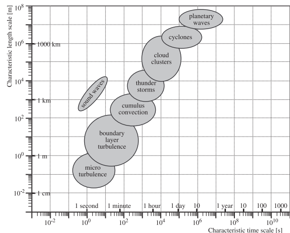
Fig. 1. Scales in the atmospheric dynamics.
