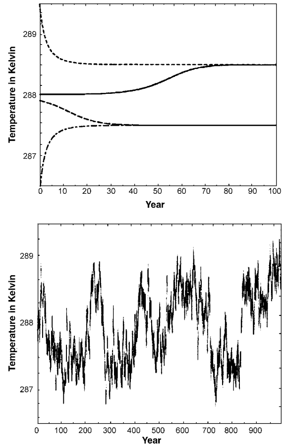
Fig. 2. (a) EBM without noise, (b) with noise.
